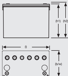
XL12V50
