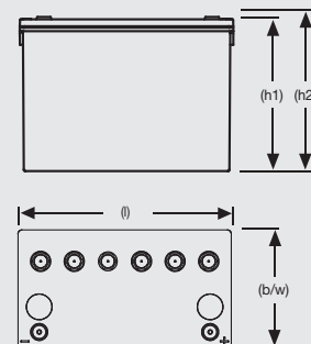
XL12V85
